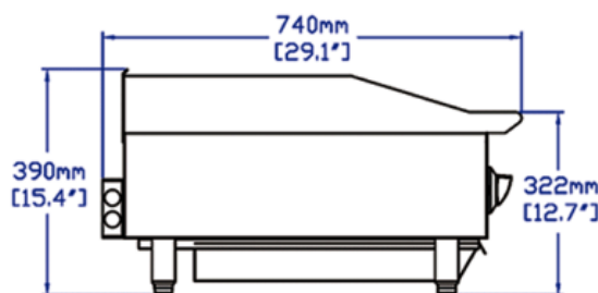
SR-EG36 SIDE VIEW
